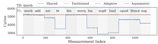
Figure 6: Covert Channels between a Spy (T0) and a Trojan (T1) Thread. In a fully shared pipeline the instructions executed on T1 have a clear effect on T0’s execution time. Partitioned , Adaptive and Asymmetric are always constant and share the same straight line.
